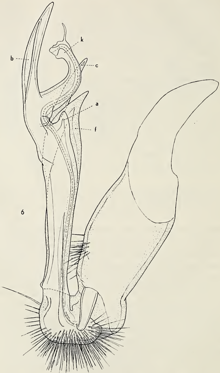
Fig. 6. Pogonosternum nigrovirgatum (Carl). — right gonopod of ♂, mesal view; a , b and c : tibiotarsal (?) processes of the acropodite; f : femoral process; k : solenomerite.
